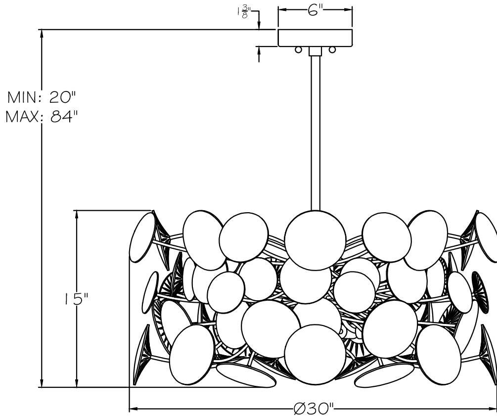
FRONT VIEW
