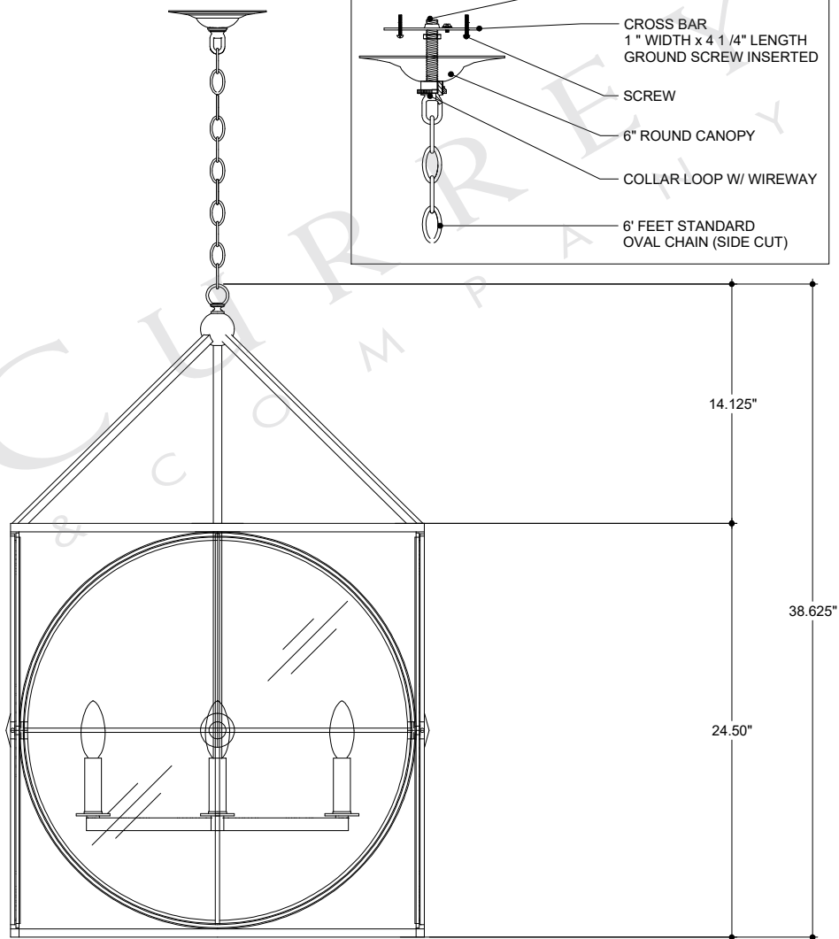
FRONT VIEW
