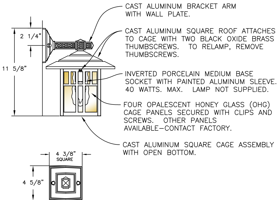
FRONT VIEW OF BRACKET ARM AND WALLPLATE
