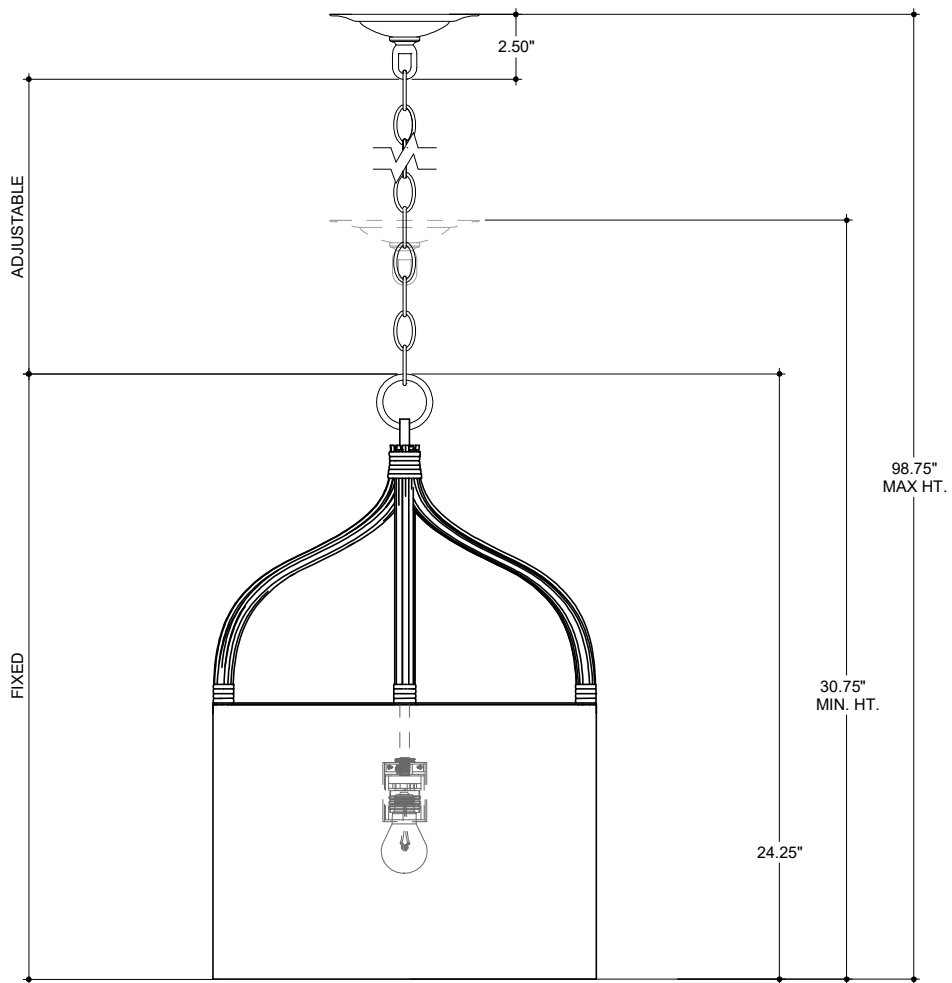
FRONT VIEW
