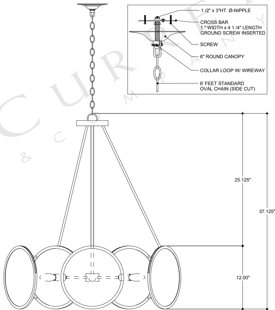
FRONT VIEW
