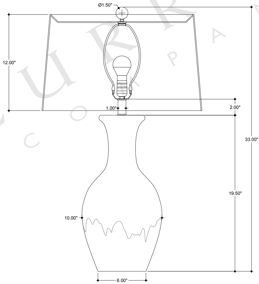
FRONT VIEW
