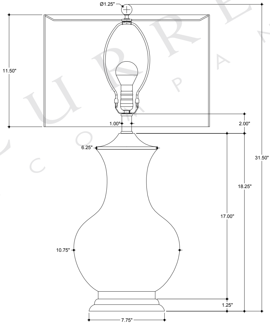
FRONT VIEW
