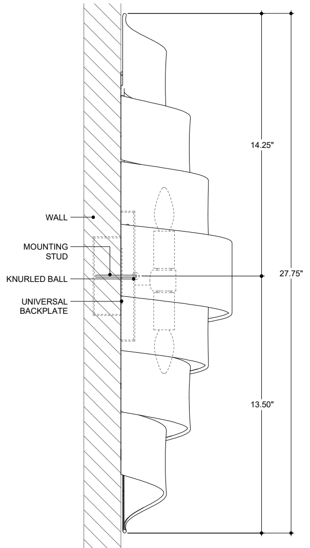
SIDE VIEW
