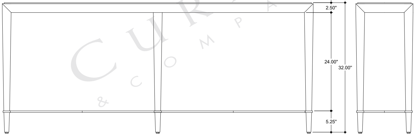
FRONT VIEW
